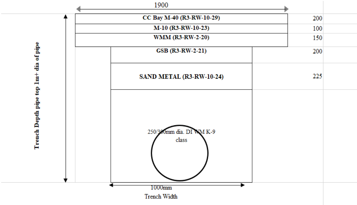
Typivcal Cross Section of Trench For Laying of 250mm & 300mm dia. DI WM in Cement concrete
