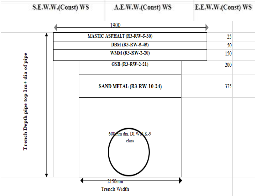
Typical Cross Section of Trench For Laying of 600mm dia. DI WM in Mastic Asphalt
